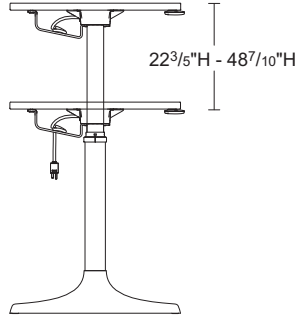
Extended Height
