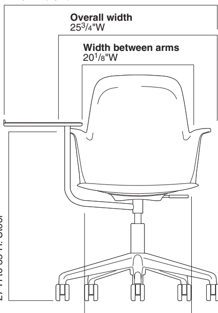
Overall width with personal workspace 29"W to 34 1 / 2 "W
