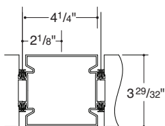
Two-Way 180°
