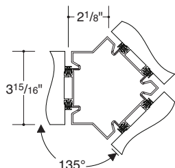
Three-Way 135°
