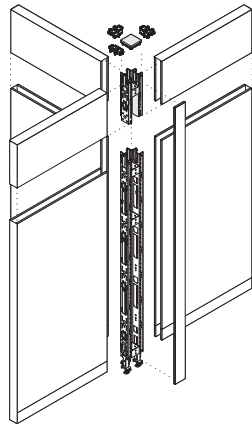
T-stacking junction includes junction and fork connectors. Full height trim, junction cap and aligner(s) must be specified separately.
