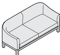
Overall: 30"D 72"W 31"H Inside: 20 3/4"D 61"W 14"H Seat: 17"H Arm: 26"H
