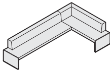
Overall: 69¼"D 123¼"W 31"H Seat: 19"D 18½"H
