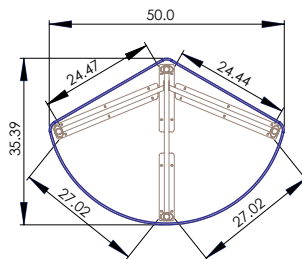
Model SS03011 Bottom View
