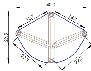
Model SS03002 Bottom View
